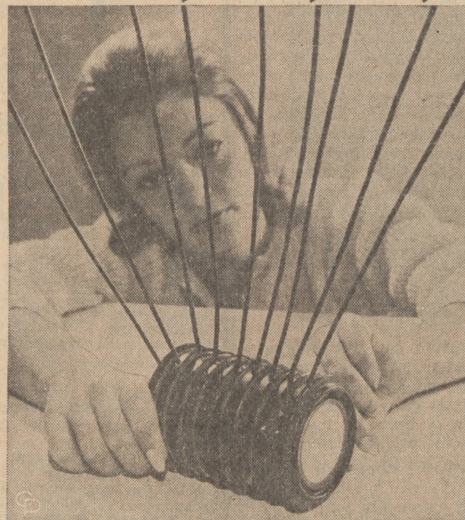
BRINGS THE STARS CLOSER—Carolyn Zamrycki looks at a new RCA image intensifier tube that makes it possible for smaller telescopes to rival the unaided viewing capability of the largest. For example, a 60-inch reflector telescope using the new tube can photograph star images now only seen with 180-inch-diameter telescopes. The National Science Foundation will allocate the new tubes to observatories around the world.
