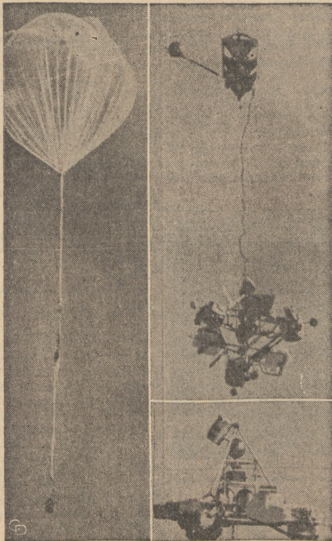
LUNAR LANDING—A test model of the Surveyor lunar soft landing spacecraft is shown during a test soft landing at Alamogordo, N.M. It dangles from the balloon (left) which carried it up 1,000 feet, begins its powered descent (upper right), and is about to touch down (lower right) on desert.
