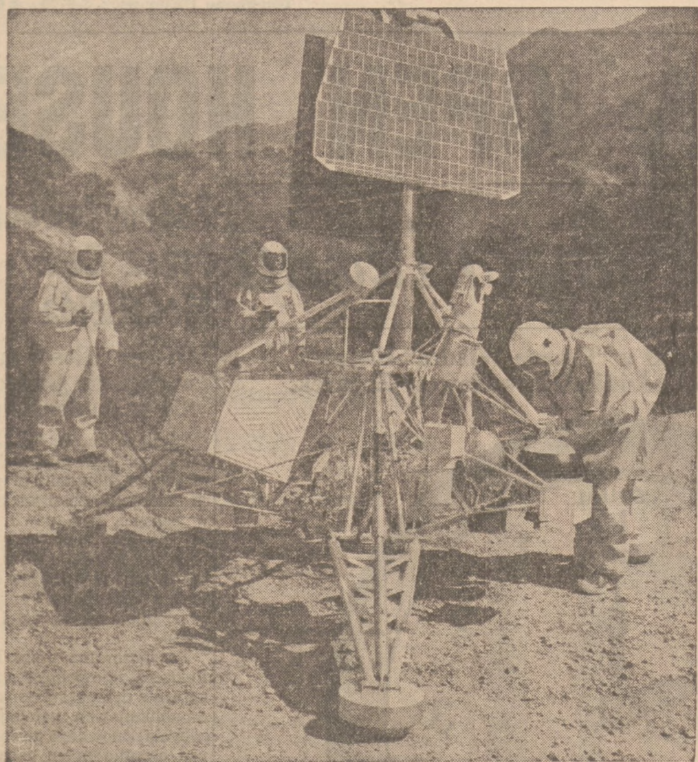
TEST SURVEYOR 2 — High in the San Gabriel Mountains in California, Hughes Aircraft technicians test a Surveyor 2 model to check performance of the vernier engine system which will lower the spacecraft gently to the Moon's surface. Surveyor 1, on the Moon since last spring, sent back more than 11,000 photos of the Moon's surface.
